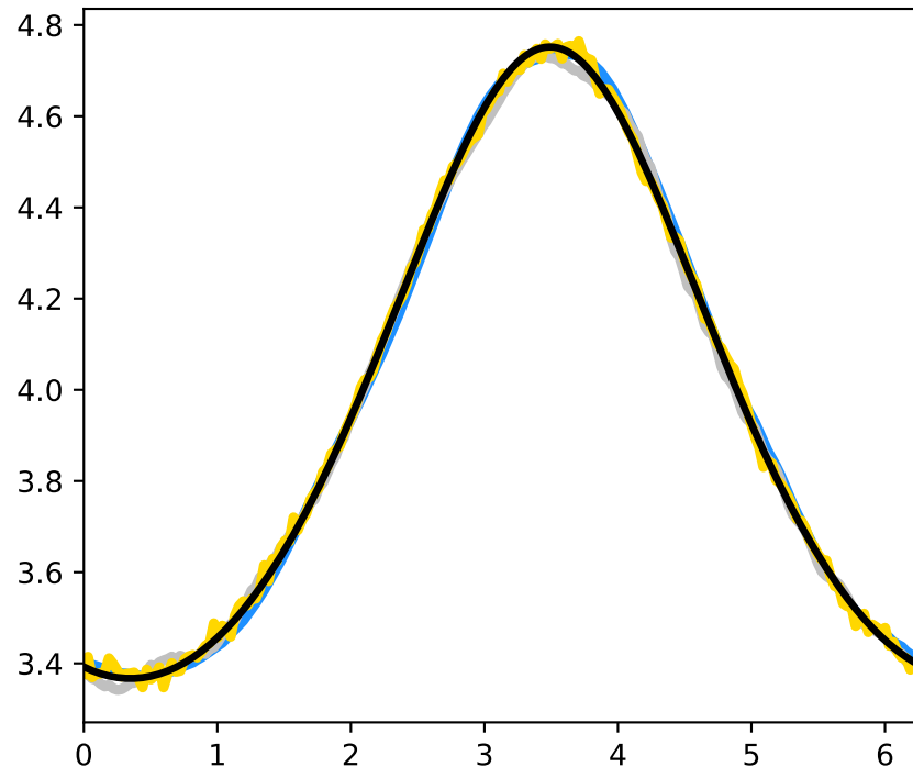
Mean State at T = T_f
