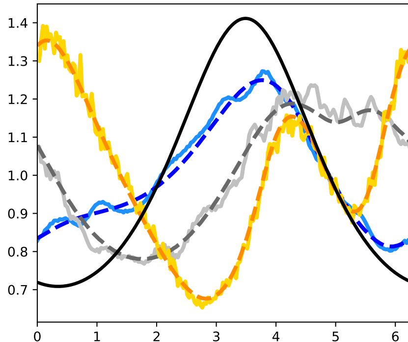
Variance and Covariance Diagonals at T = T_f
